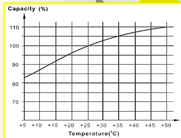
TEMPERATURE vs CAPACITY
