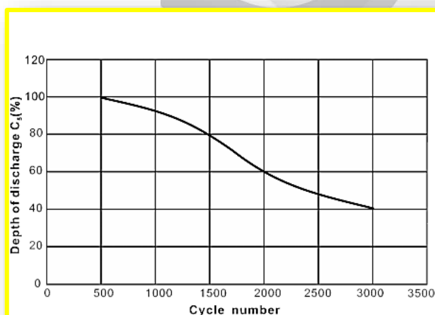
CYCLES vs D.O.D
